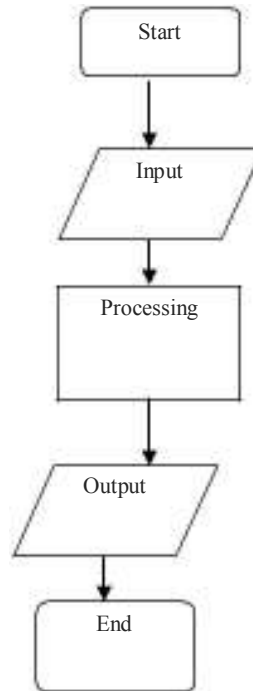
Figure 9: Flow chart
