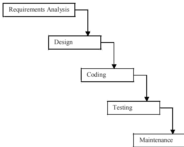
Figure 1: Waterfall model
