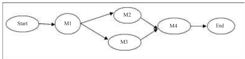
Figure 4: Flow graph
